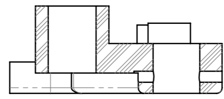
SECTION X-X
